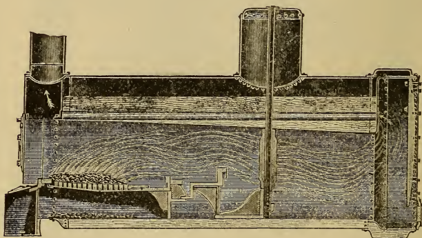
FIG. 40.—THE "HUBER" BOILER.
